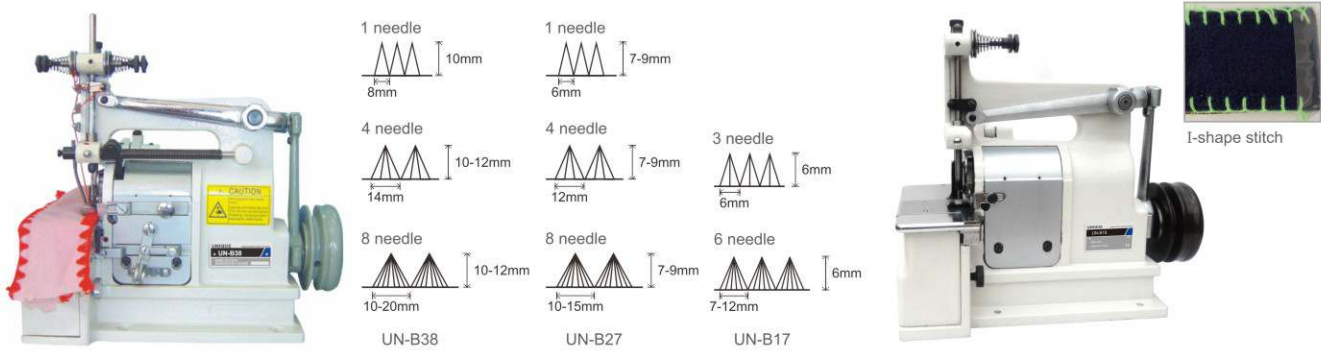
UN-B38 Shell stitch overlock sewing machine UN-B38 Big shell 1, 4, 8 stitches UN-B27 Medium shell 1, 4, 8 stitches UN-B17 Small shell 1, 3, 6 stitches
