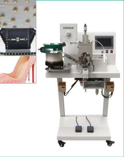
UN-198-9 Automatic four claws base button plastic pearl nail attaching machine
