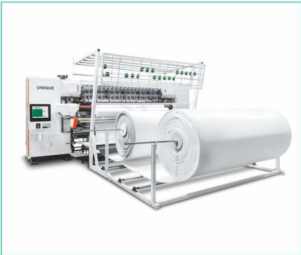
UN-Q3200B High-speed computerized chain stitch multi-needle quilting machine Quilting width 2450mm 3 needle rows with 3"+3" inch between needle bars
