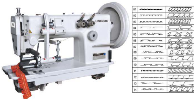
UN1260G Multi-function chainstitch gathering machine
