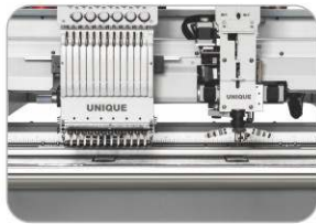
UN-F901+1PQ Special embroidery machine for flat, coiling and taping
