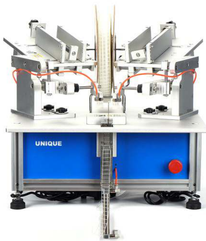
UN-TM7002 Automatic 2-head lable staple attaching machine for clothes tagging
